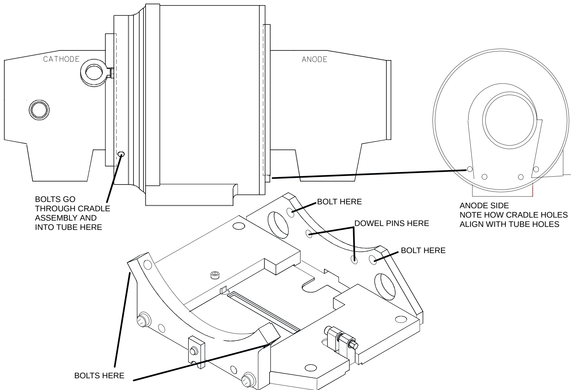
FIGURE 50 CRADLE ASSEMBLY
