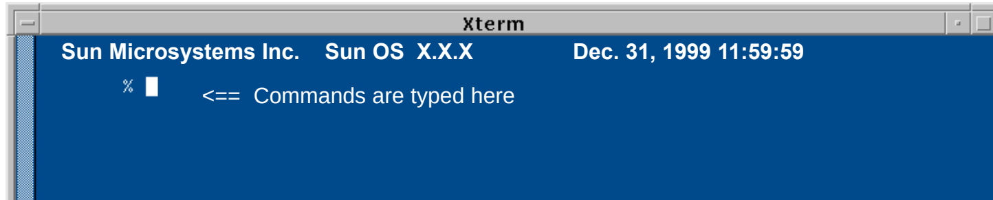
FIGURE 146 Xterm Window
