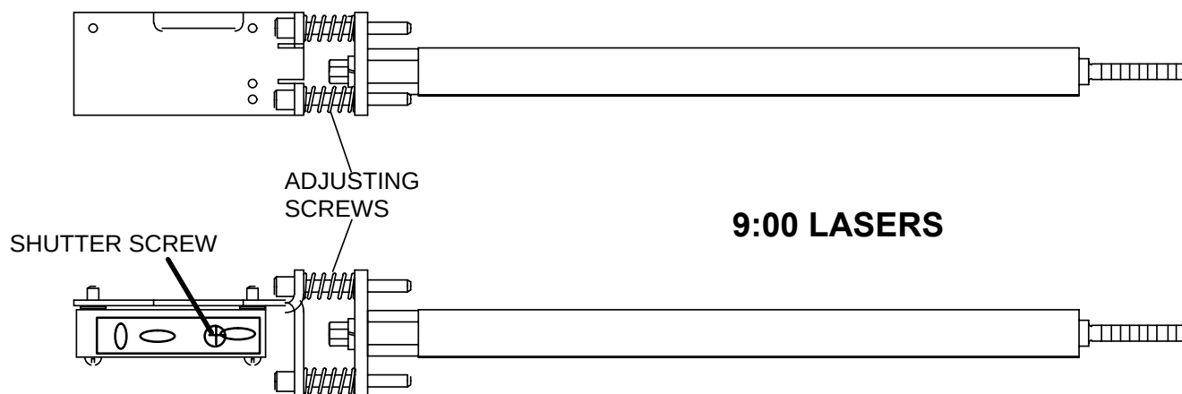
FIGURE 91 LASER ALIGNMENT SCREWS
