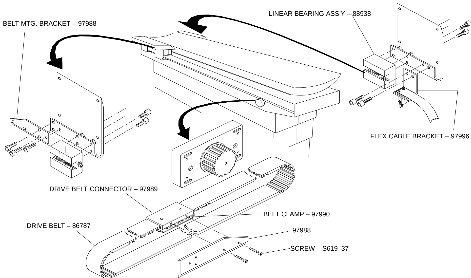
FIGURE 160 PATIENT SUPPORT ASSEMBLY - 171850A
