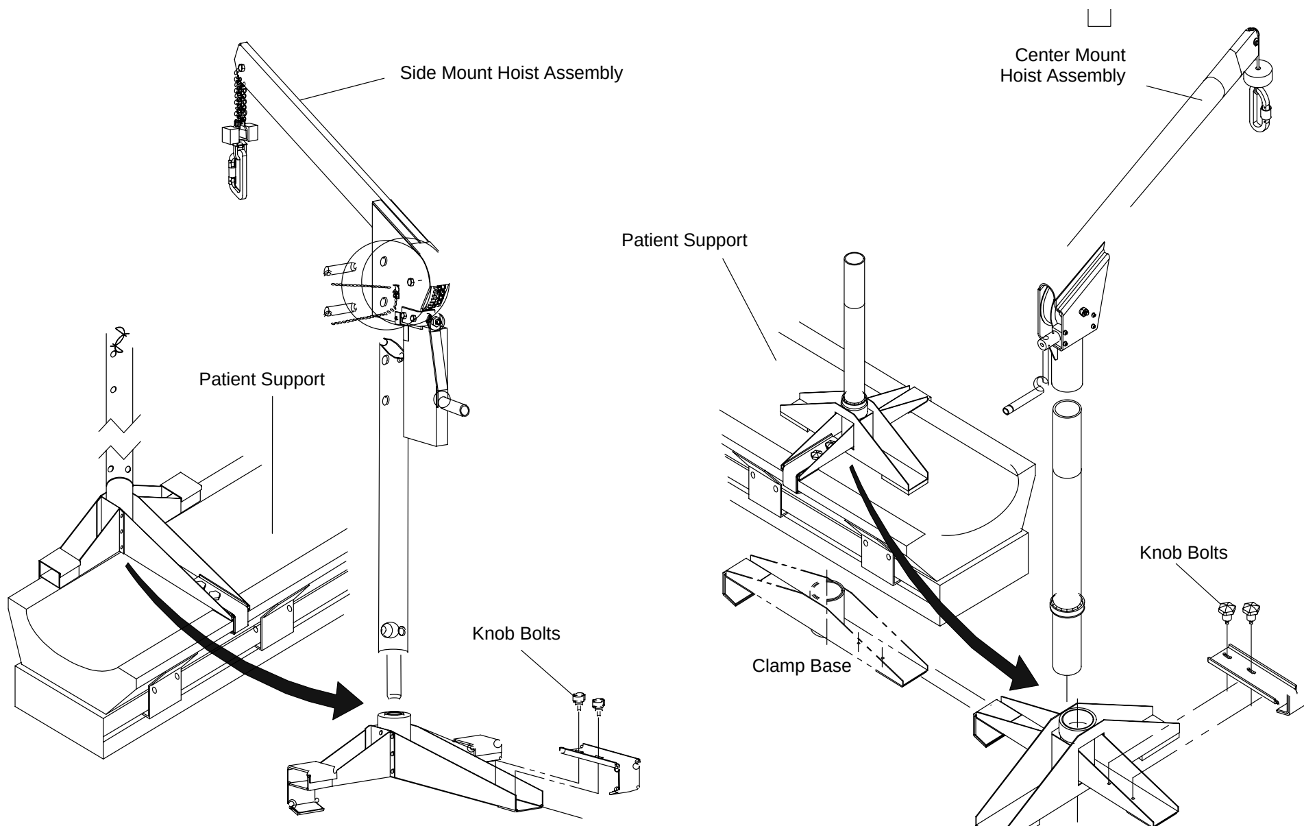
FIGURE 249 HOIST ASSEMBLY
