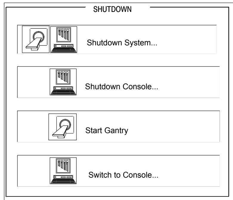
FIGURE 327 SHUTDOWN SCREEN
